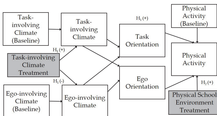
FIGURE 5 Path model presenting the theorized relationships between the variables and treatment effects (Study IV).
