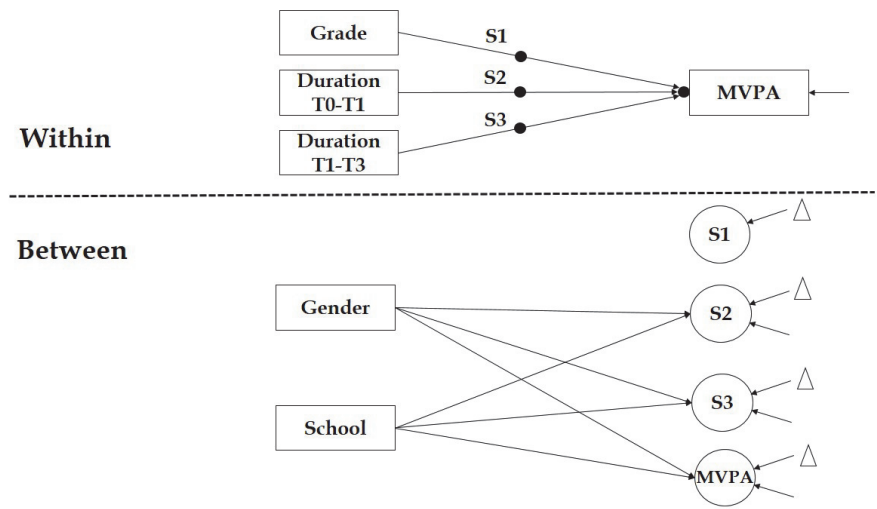
FIGURE 3 The two-level regression model of self-reported MVPA with intercept and random regression coefficients.
